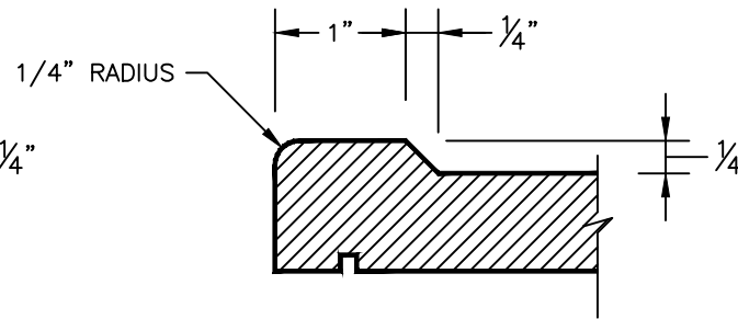
STANDARD MARINE EDGE EPOXY RESIN COUNTERTOP W/ 1/4" MACHINED RADIUS EDGE & DRIP GROOVE (1" & 1-1/4" THICK TOPS AVAILABLE, THICKNESS AT FRONT EDGE)
