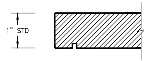
STANDARD FLAT EPOXY RESIN COUNTERTOP W/ EASED EDGE BREAK & DRIP GROOVE (3/4", 1" & 1-1/4" THICK TOPS AVAILABLE)
