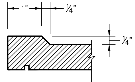
STANDARD MARINE EDGE EPOXY RESIN COUNTERTOP W/ EASED EDGE BREAK & DRIP GROOVE (1" & 1-1/4" THICK TOPS AVAILABLE, THICKNESS AT FRONT EDGE)
