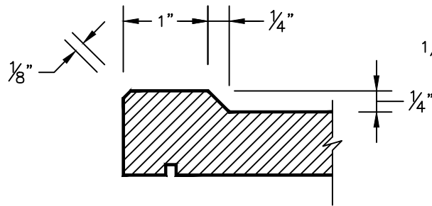
STANDARD MARINE EDGE EPOXY RESIN COUNTERTOP W/ 1/8" BEVEL EDGE & DRIP GROOVE (1" & 1-1/4" THICK TOPS AVAILABLE, THICKNESS AT FRONT EDGE)
