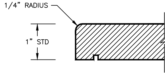
STANDARD FLAT EPOXY RESIN COUNTERTOP W/ 1/4" MACHINED RADIUS EDGE & DRIP GROOVE (3/4", 1" & 1-1/4" THICK TOPS AVAILABLE)
