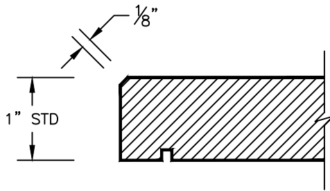
STANDARD FLAT EPOXY RESIN COUNTERTOP W/ 1/8" BEVEL EDGE & DRIP GROOVE (3/4", 1" & 1-1/4" THICK TOPS AVAILABLE)
