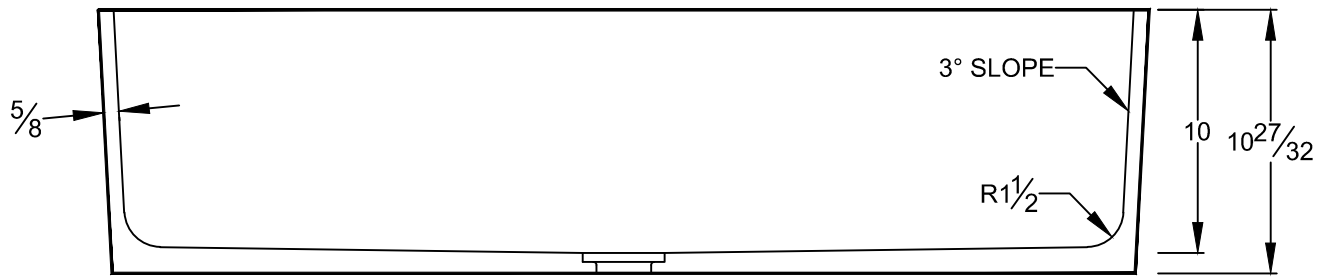
SECTION VIEW
