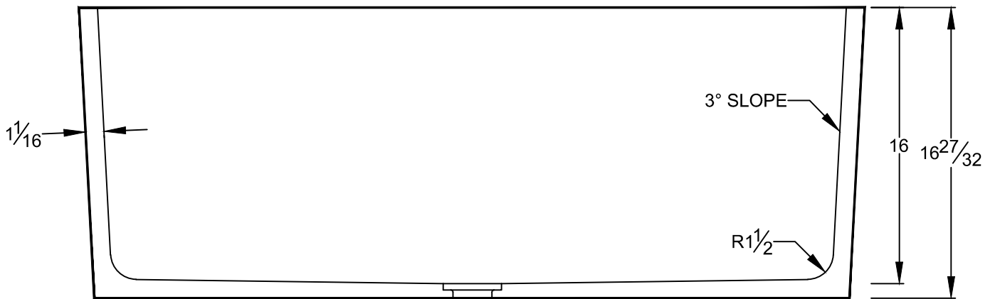
SECTION VIEW
