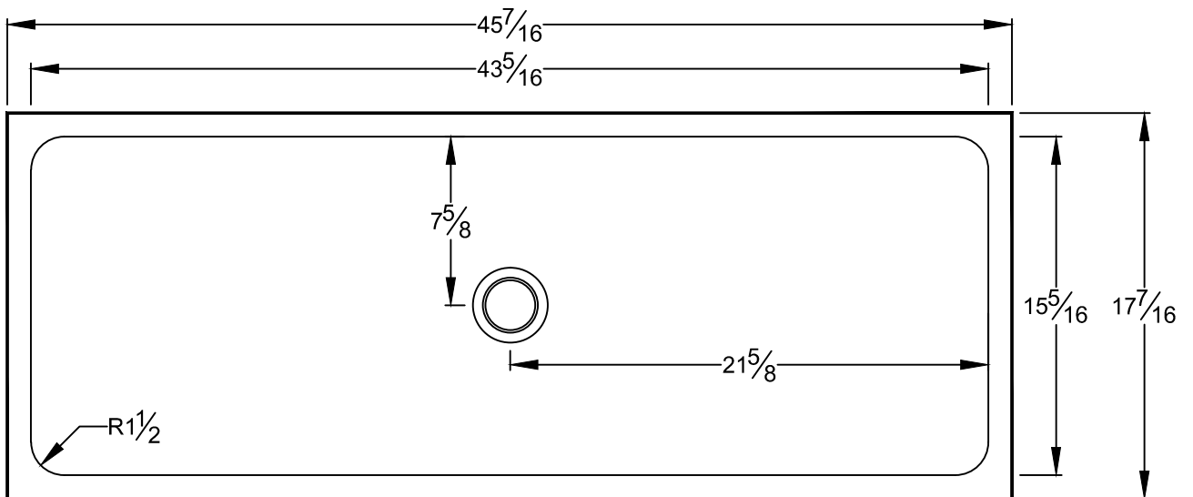
TOP VIEW
