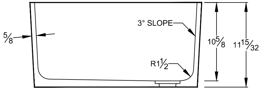
SECTION VIEW
