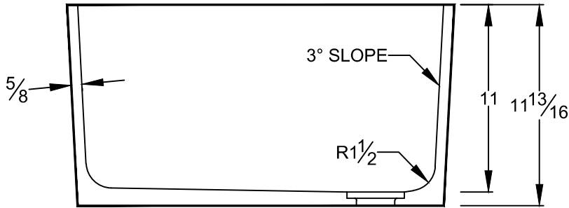
SECTION VIEW
