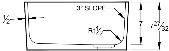
SECTION VIEW
