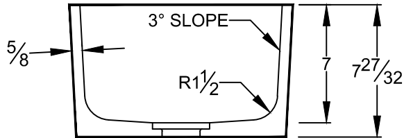
SECTION VIEW
