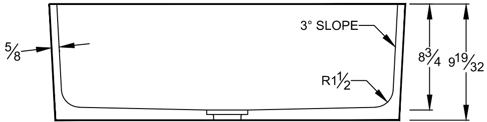
SECTION VIEW
