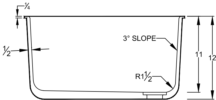
SECTION VIEW
