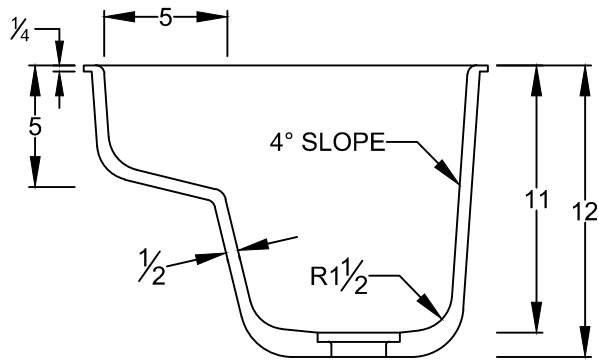
SECTION VIEW (FRONT TO BACK)
