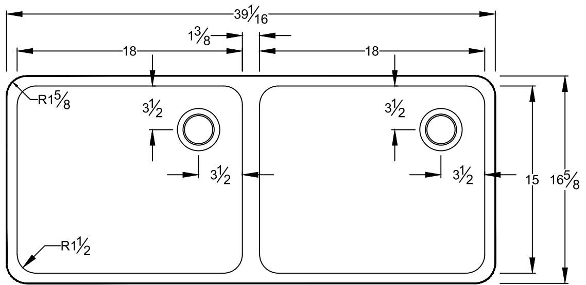
TOP VIEW
