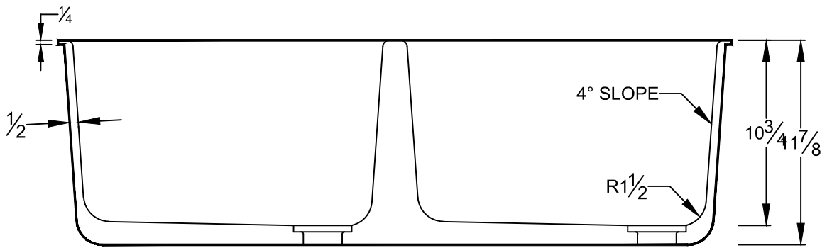
SECTION VIEW
